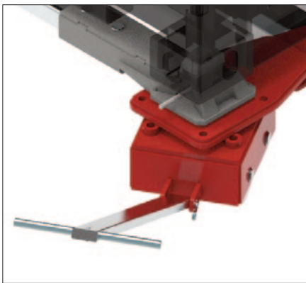
Rotation of the single wheel boxes
