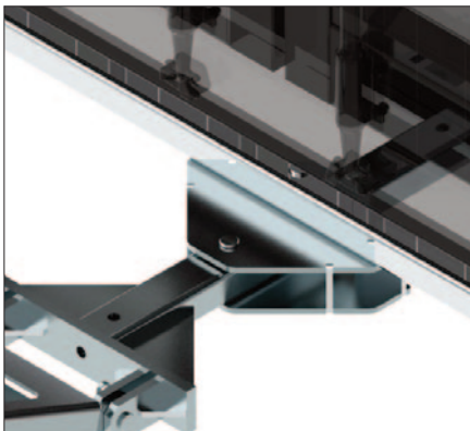
With bolts the steerable skate becomes a fixed rear skate
